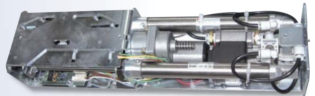
Compressed Air Generator „One Air Blast“ (Encapsulated Maintenance-Free System)
